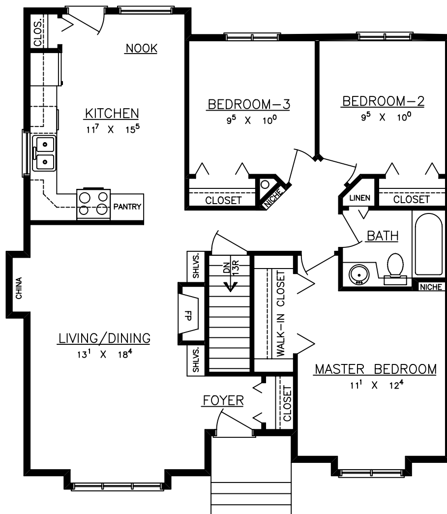
FLOOR PLAN
